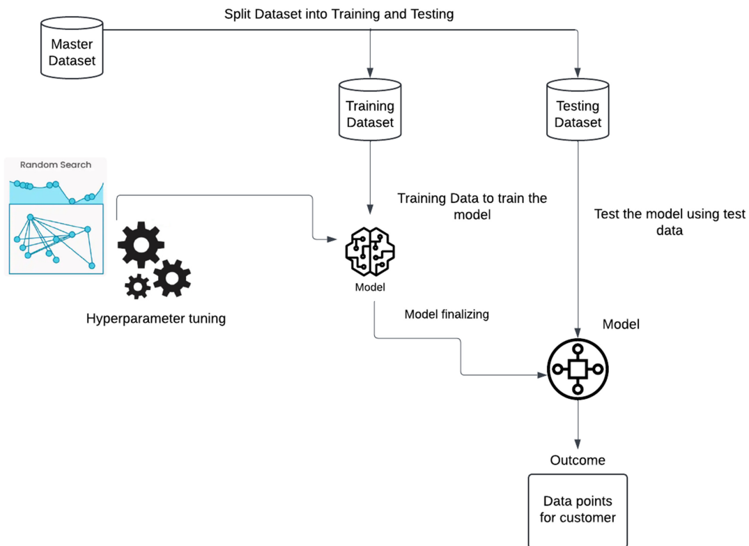
Figure 2 Hyperparameter optimization
