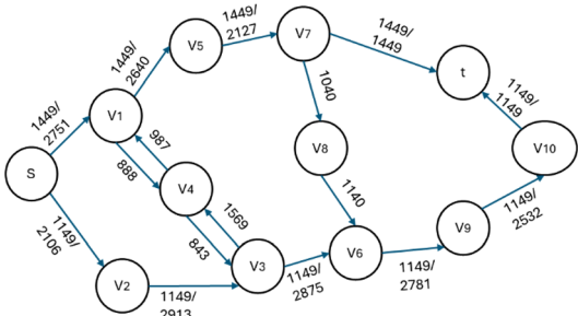
Figure 8 Weighted directed graph according to the total capacity PCU
