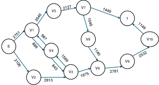
Figure 9 Ford–Fulkerson algorithm results
