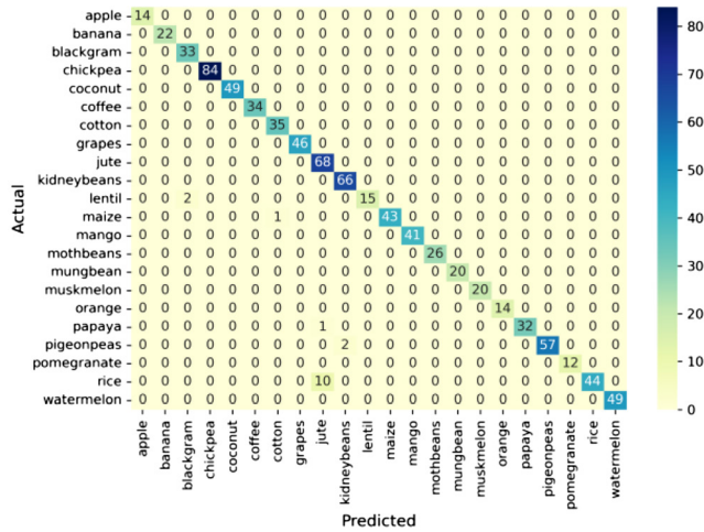
Classification output of the KNN algorithm
