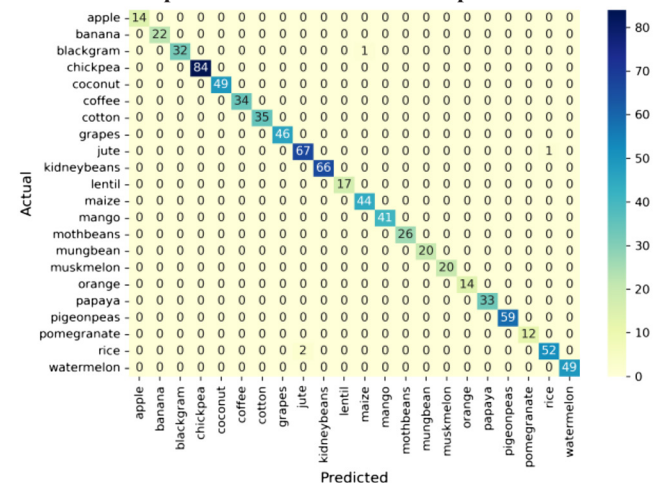
DT predictions versus actual crop classes
