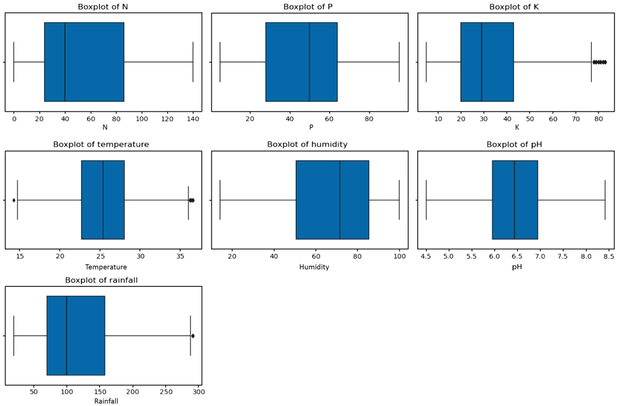
Figure 14 Outcomes for boxplots in the proposed method
