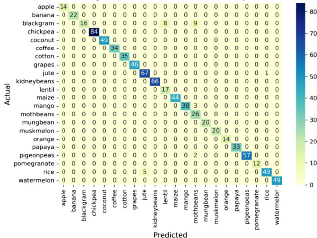
True and predicted classifications using GNB
