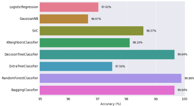
Accuracy performance of different ML classifiers
