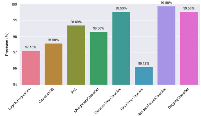
Precision of the different ML classifiers
