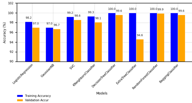
Outcomes of the accuracy of the proposed method
