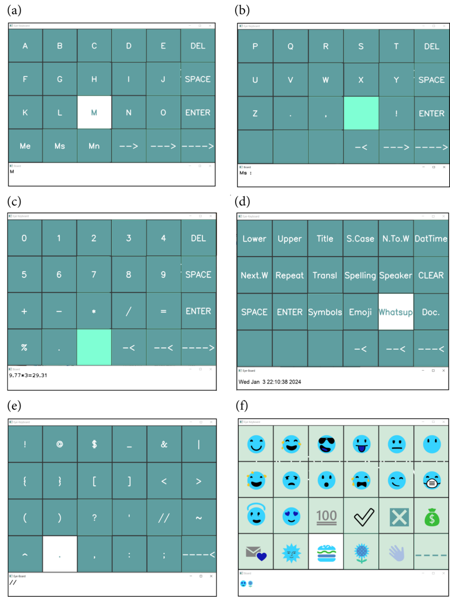
Figure 1 Visualization of the virtual keyboard
