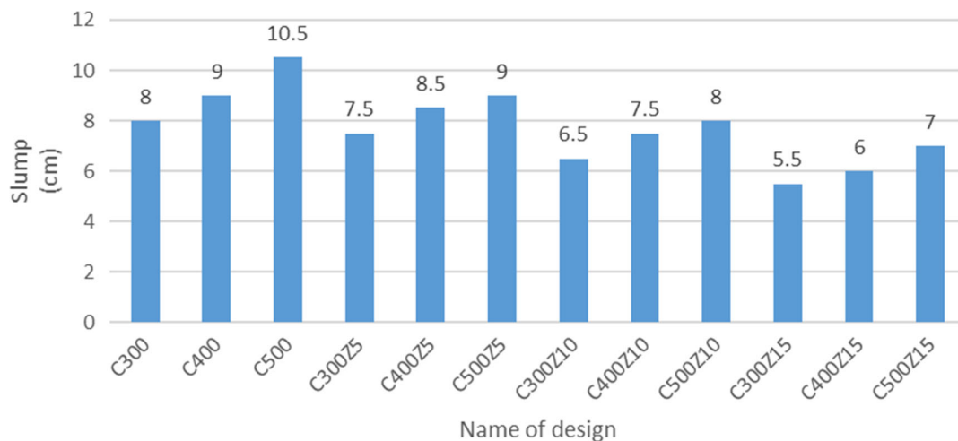
Figure 3 Slump test results for all designs
