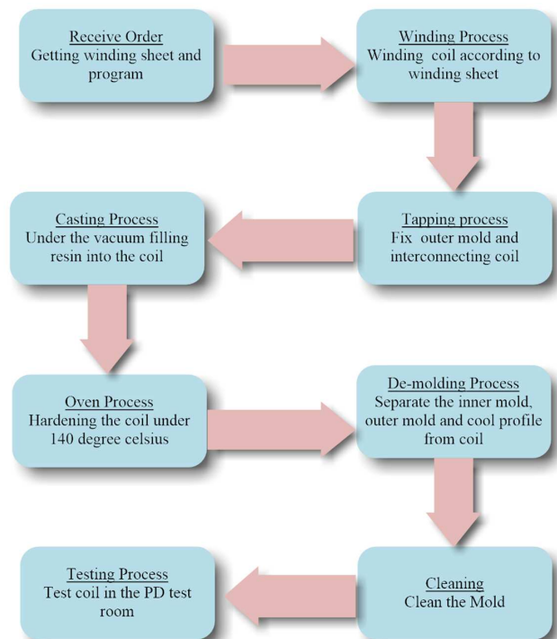
Figure 2 Manufacturing process of power transformer at Asia Trafo LLP in Shymkent, Kazakhstan
