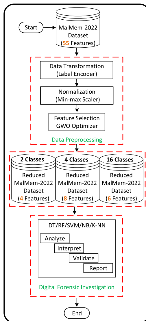
Figure 3 The DFI model
