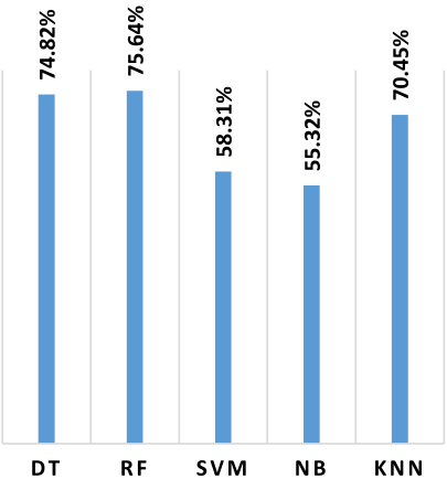
Figure 6 Recall of the DFI model with 16 classes
