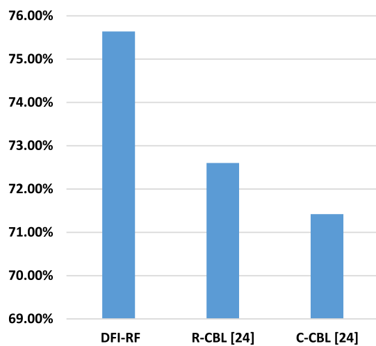
Figure 10 The DFI-RF model accuracy versus other forensic models using CIC-MalMem-2022 dataset (16 classes)
