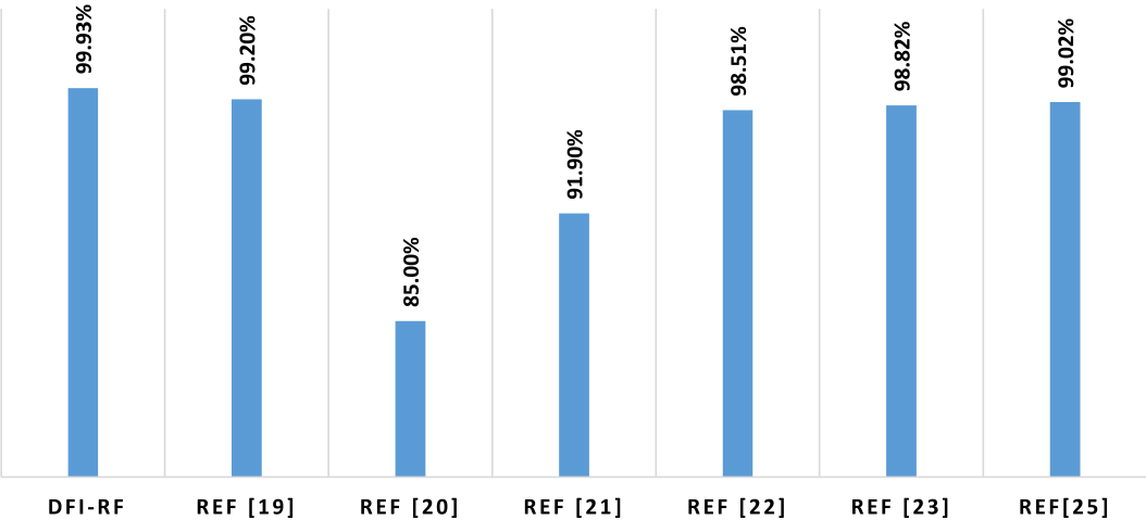
Figure 8 The DFI-RF model accuracy versus other forensic models across several datasets (binary classification)
