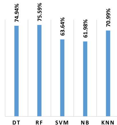
Figure 5 Precision of the DFI model with 16 classes
