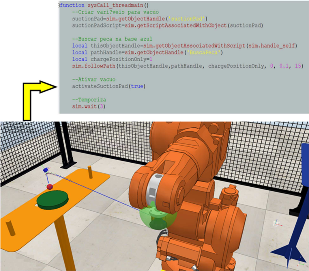
Figure 3 Real programming of the robot after validation of the virtual system
