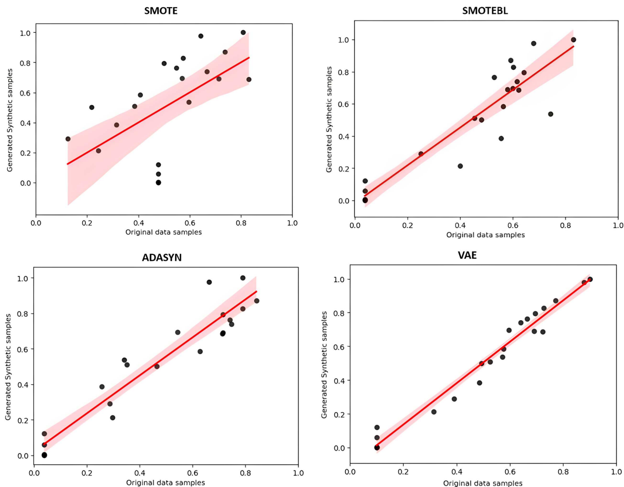
Figure 5 Performance comparison of VAE against other DA schemes using scatterplot
