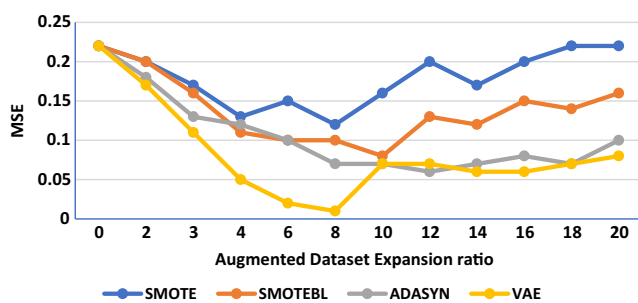
Figure 6 Performance comparison of different DA schemes against expansion ratio
