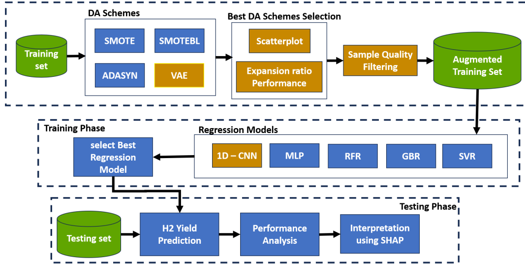
Figure 2 The proposed VAE-CNN model schematic design with its control flow
