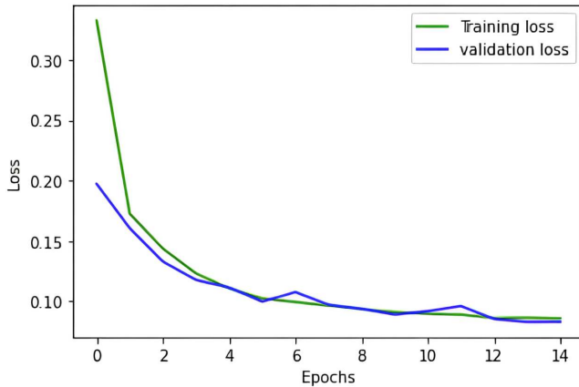
Figure 4 Learning curve of VAE in DA process
