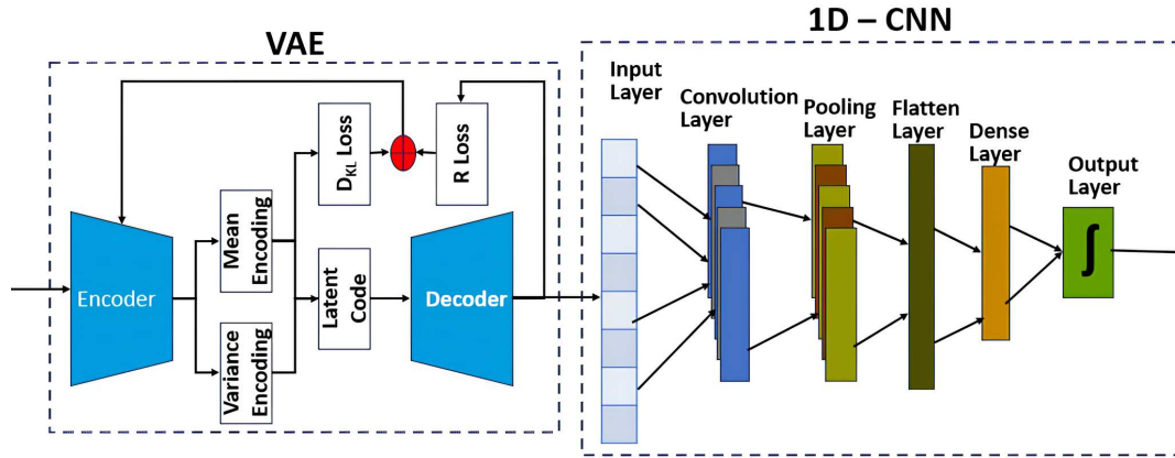
Figure 2 The proposed VAE-CNN model schematic design with its control flow
