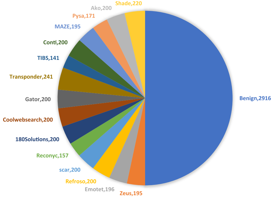
Figure 4 Malware breakdown
