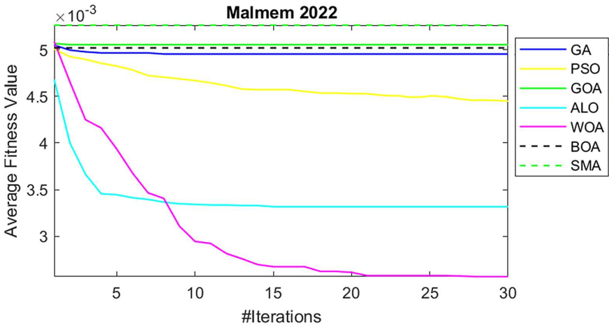
Figure 5 Comparison of fitness values
