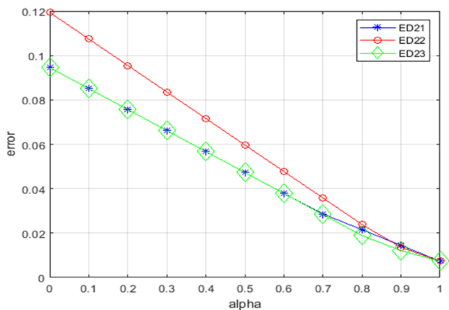
Figure 4 Errors at t = 1 - H 2 - differentiable in the second form
