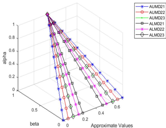
Figure 3 Approximations - H 2 - differentiable in the second form
