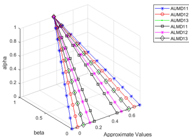
Figure 1 Approximations - H_2 -differentiable in the first form
