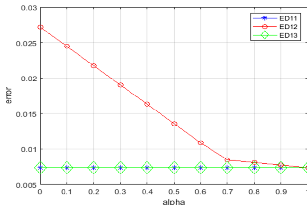
Errors at t = 1 - H_2 -differentiable in the first form
