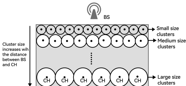
Figure 1 Unequal clustering architecture in WSN
