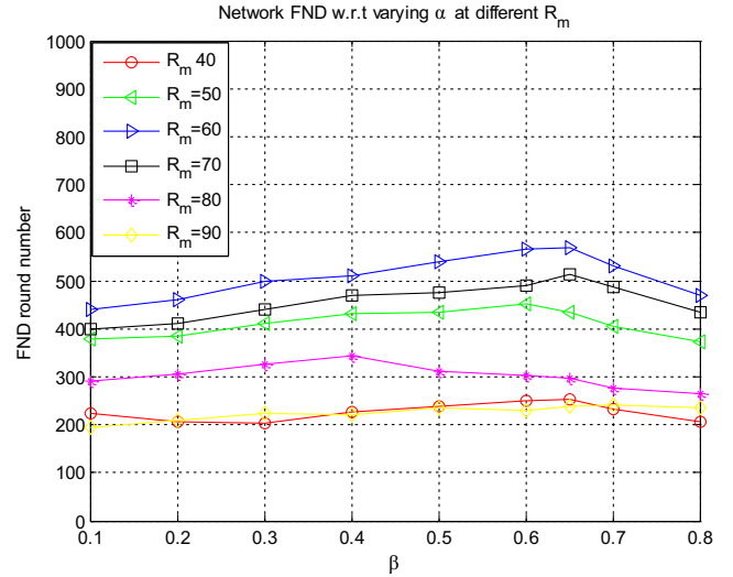
Figure 8 FND metric of suggested network setup for different R_m
