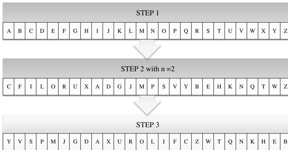
Figure 6 Steps for encrypting a message with n = 2
