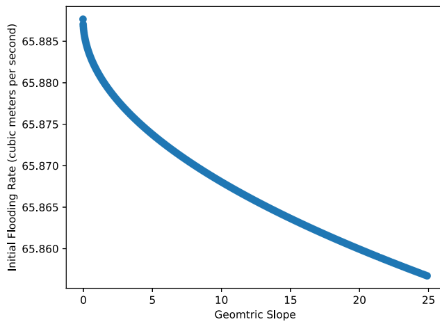
Figure 7 Plot of geometric slope v. initial flooding rate
