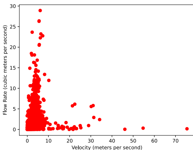
Figure 4 Plot of velocity v. flow rate for the Baltimore County storm-drain spatial dataset
