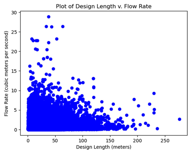
Figure 5 Plot of design length v. flow rate for the Baltimore County storm-drain spatial dataset
