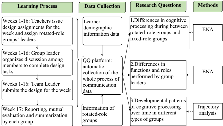
Figure 2 Research design
