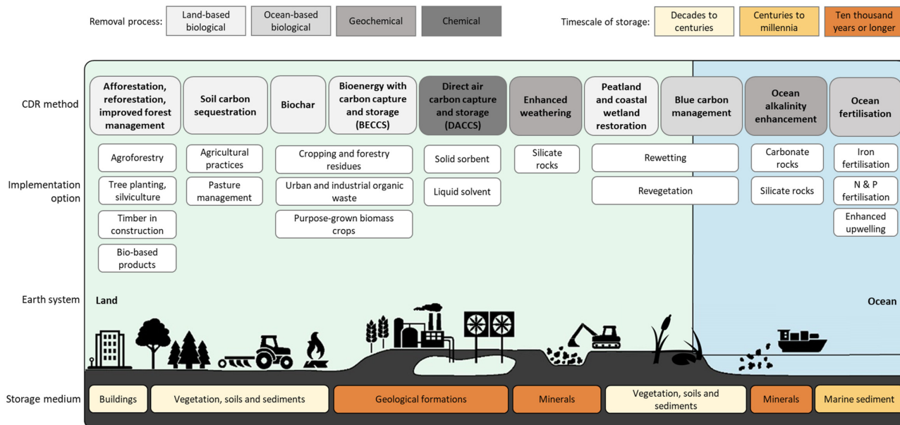
Figure 1 The taxonomy of carbon dioxide removals (CDRs)
