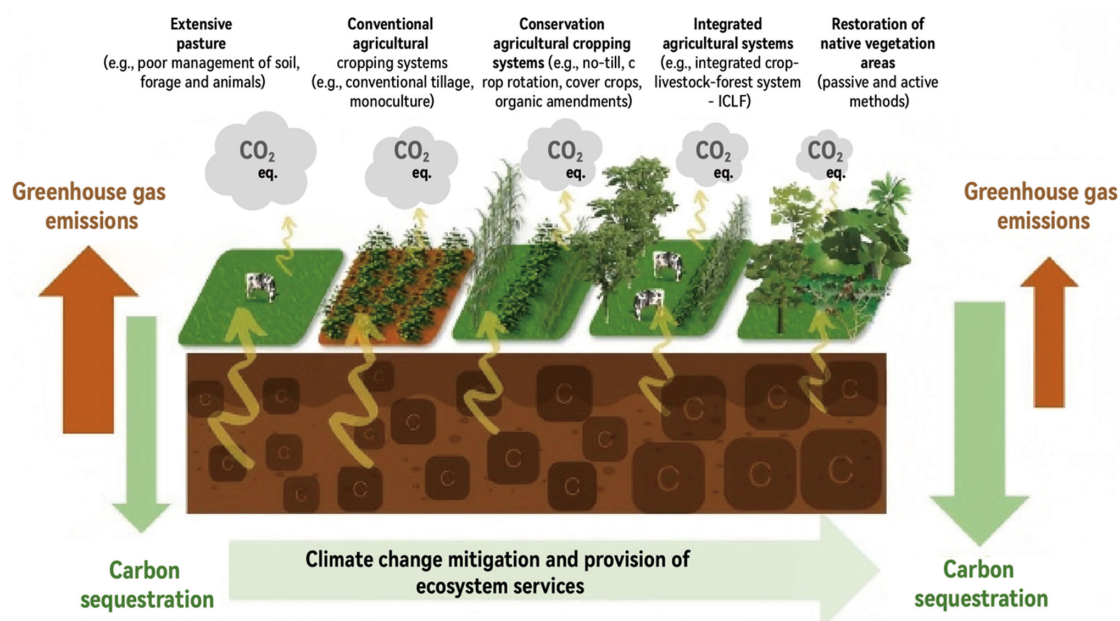
Figure 4 Pathways for a climate-smart intensification and diversification of production systems in Latin America
