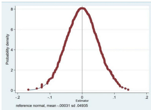
Figure 4 Placebo test
