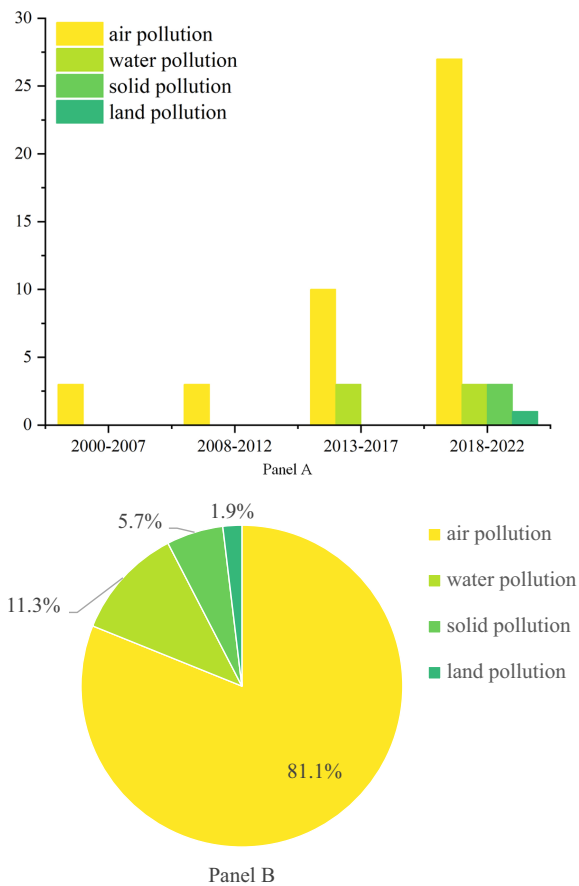
Figure 3 Pollution category ( N = 50, p = 0.503 )
