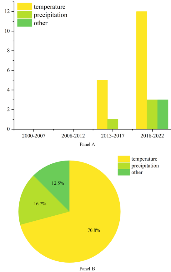
Figure 4 Climate change category ( N = 25, p = 0.410 )
