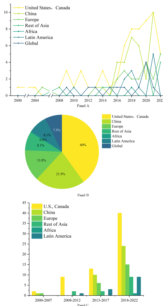
Figure 8 Research country ( N = 145 , p = 0.154 ), ( N = 46 , p = 0.011 ) 4
