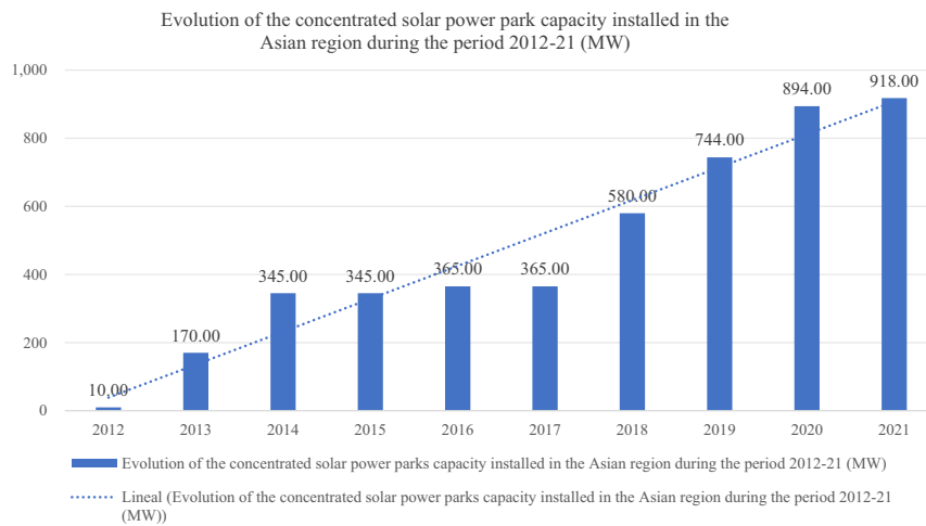
Figure 11 The development of CSP park capacity installed in Asia between 2012 and 2021
