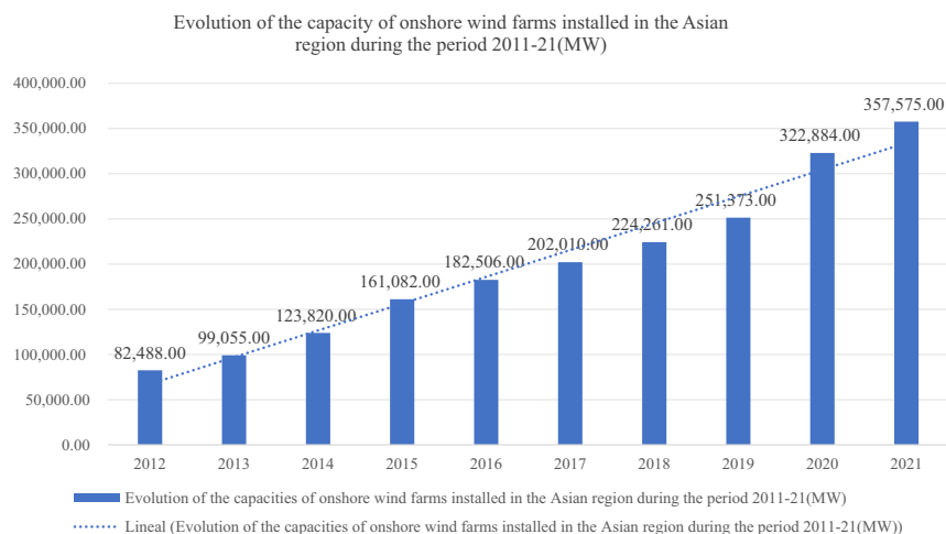
Figure 4 Changes in the installed capacity of onshore wind farms in the Asian region between 2012 and 2021
