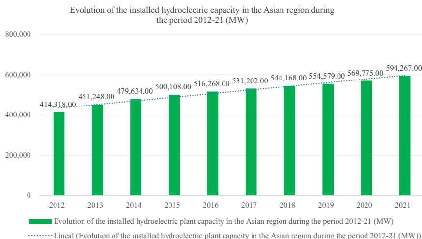
Figure 2 Reflects the changes in installed hydroelectric plant capacity in Asia from 2012 to 2021
