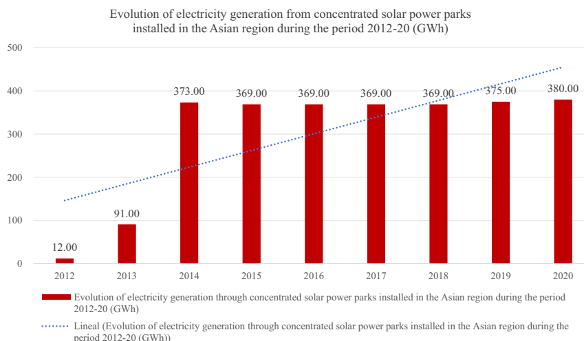
Figure 12 Evolution of electricity generation from CSP parks installed in the Asian region during the period 2012–2020
