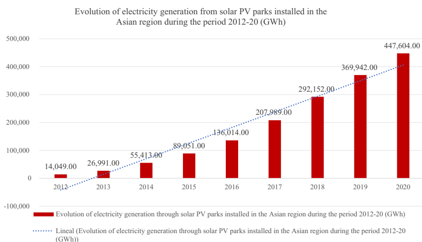
Figure 10 Development of power production from solar PV parks installed in Asia between 2012 and 2020
