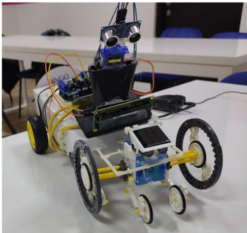
Figure 3 Hardware prototyping/production
