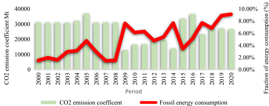
Figure 2 CO 2 emission coefficient (CEC) and fossil fuel energy share in the CHPH
