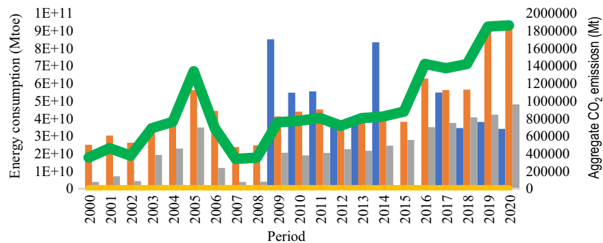
Figure 1 Energy consumption variation and CO 2 emissions of Nigeria's CHPH
