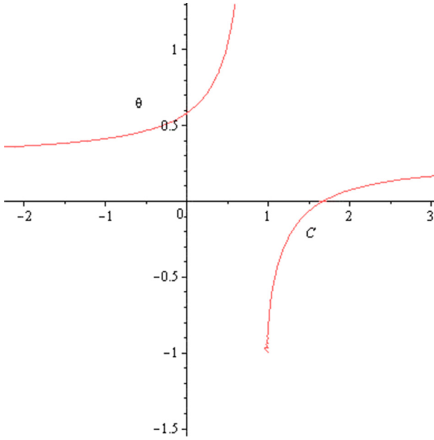
Figure 2 The Shilnikov bifurcation area
