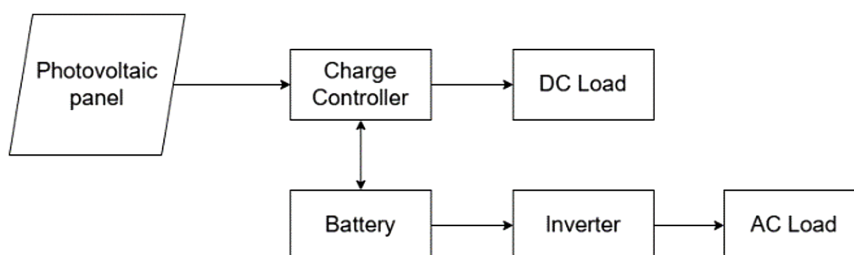
Figure 1 Block diagram of off-grid solar home system
