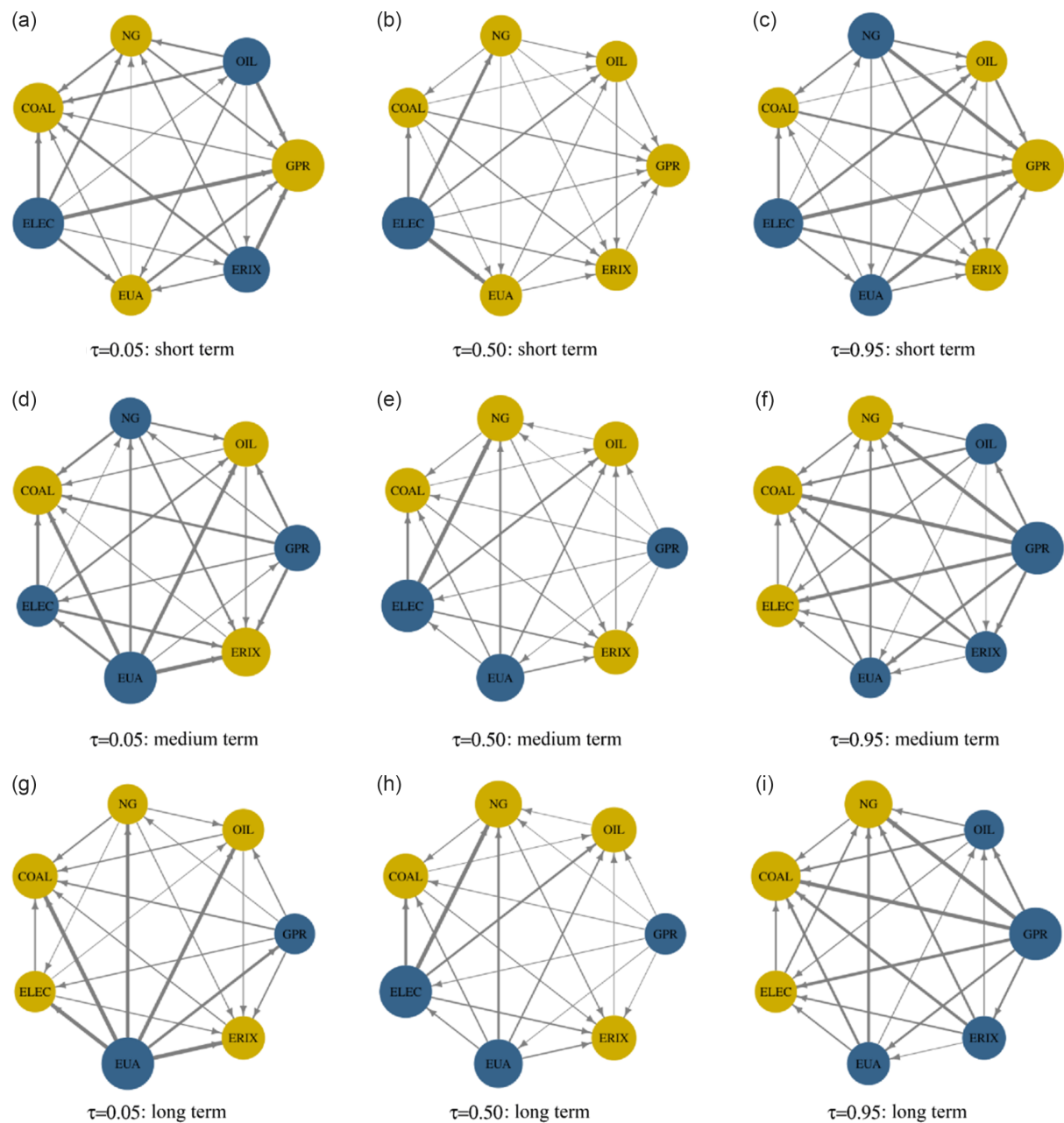
Figure 8 Time-frequency-domain connectedness networks in three quantiles
