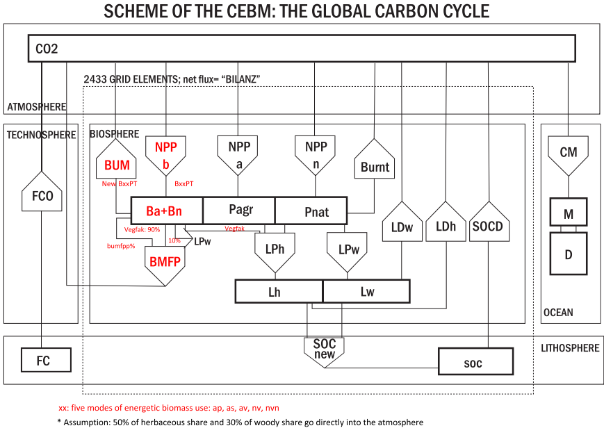
Figure 2 The structure of the global carbon reservoirs and flows in the CEBM
