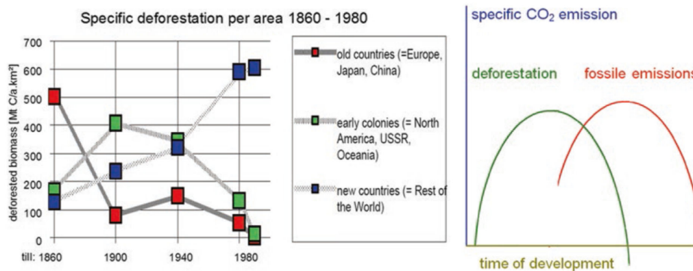
Figure 14 Historic cyclicity in global deforestation patterns. Biomass by world region according to CEBM data
