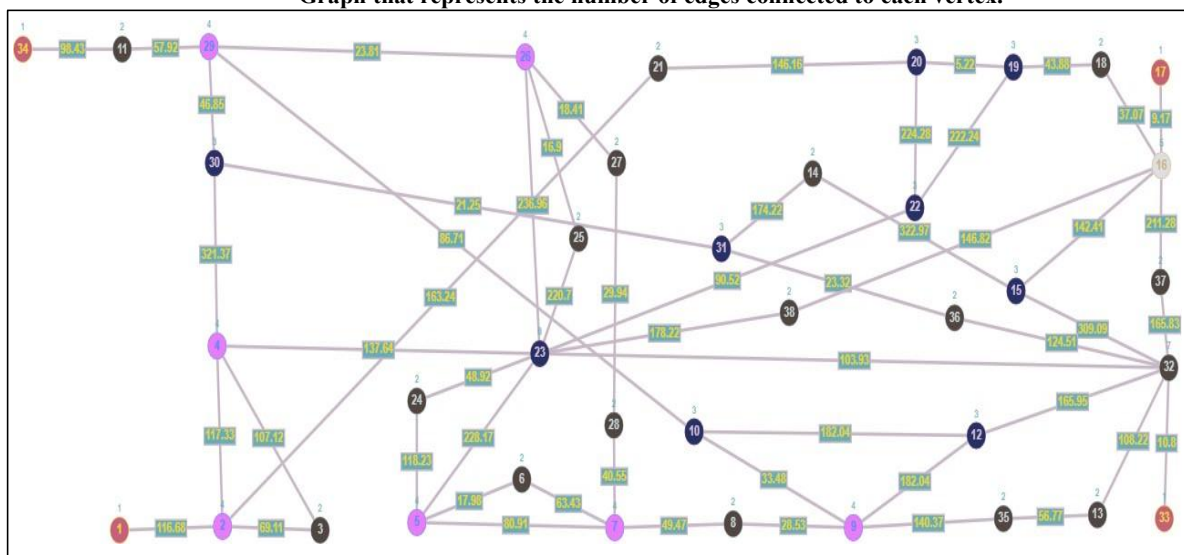
Figure 7 Graph that represents the number of edges connected to each vertex.
