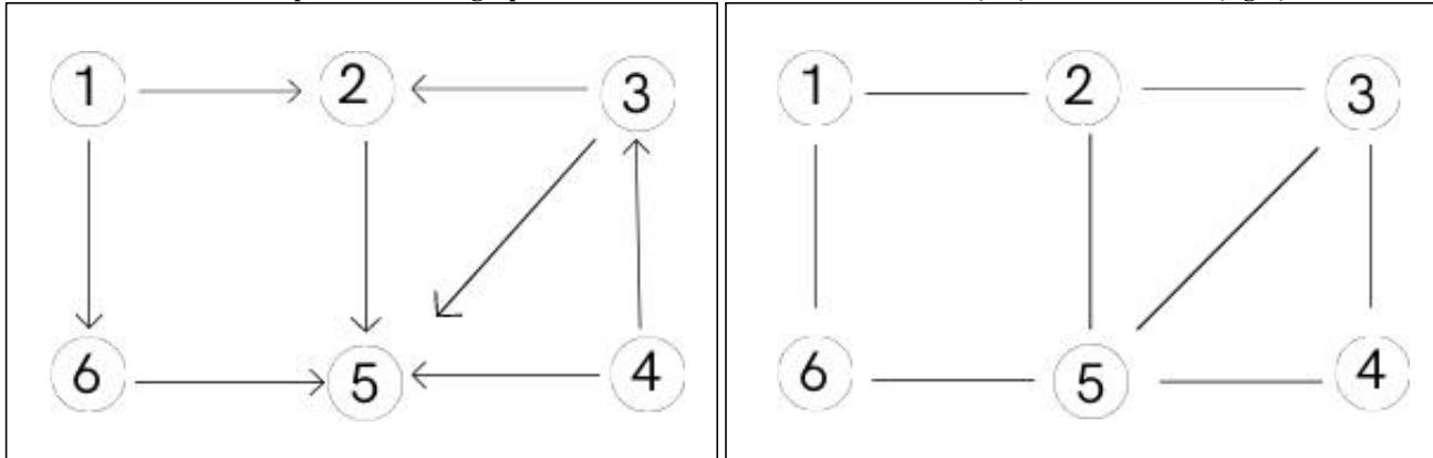
Figure 6 Representation of graphs with six vertices considered oriented (left) and unoriented (right).
