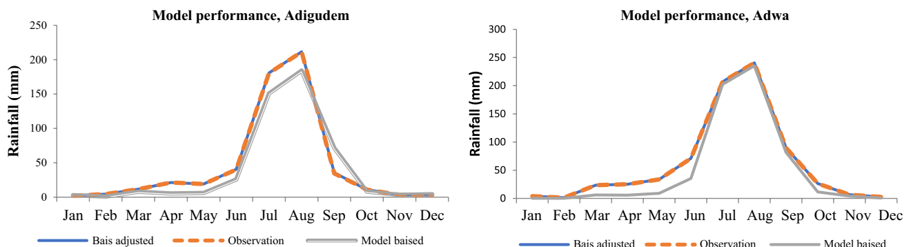
Figure 5 Model performance in simulating rainfall
