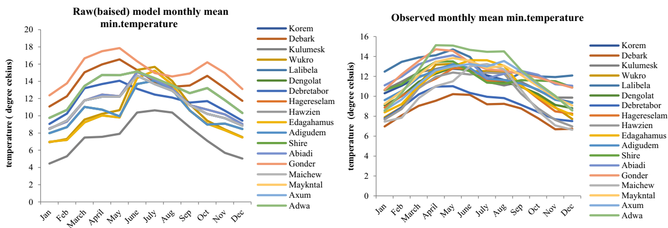
Figure 4 UTRB model ensemble raw/biased and observation data, minimum temperature
