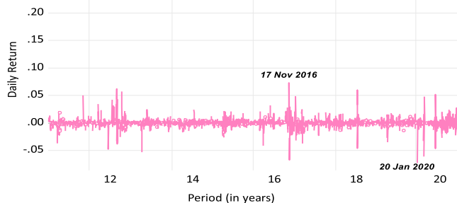
Figure 6 Ln return (wheat)
