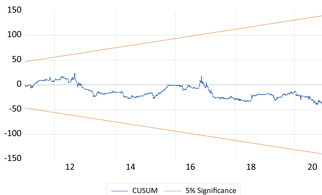
Figure 12 CUSUM plot wheat
