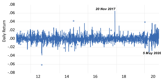
Figure 8 Ln return (soyabean)
