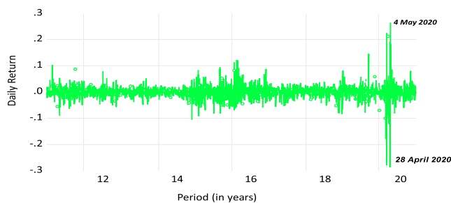
Figure 5 Ln return (crude)
