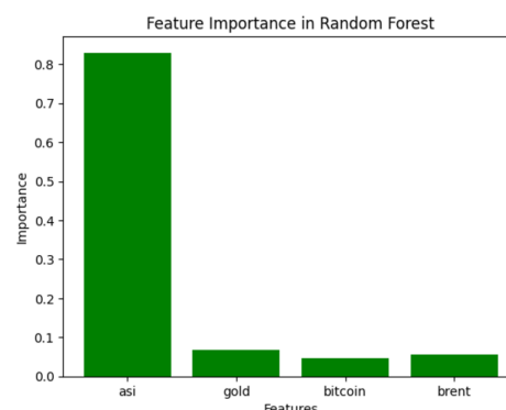
Figure 2 Random forest
