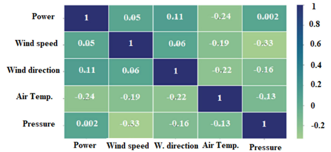
Figure 2 Correlation map between power output and climatic data
