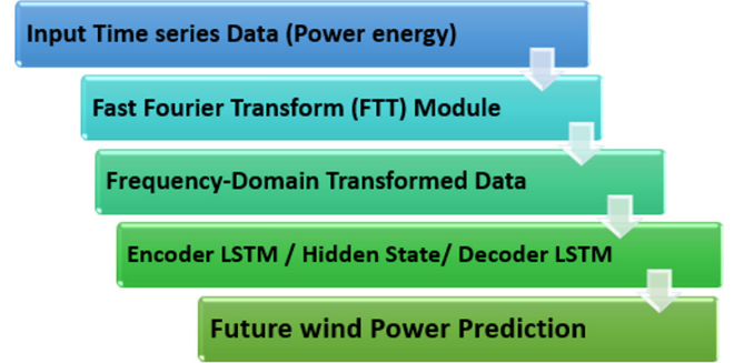
Figure 4 The proposed process of the FFT-encoder-decoder-LSTM model
