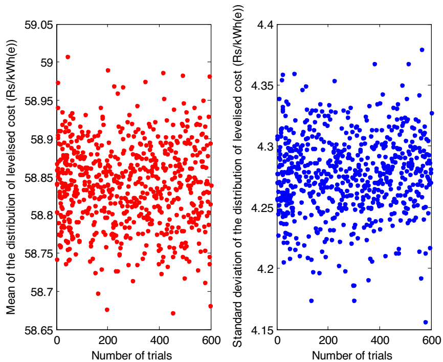
Figure 13 Sampling distributions of mean and standard deviations of levelized round trip cost of electrical energy storage (Pb-acid batteries, 1 MW, 2-h storage)
