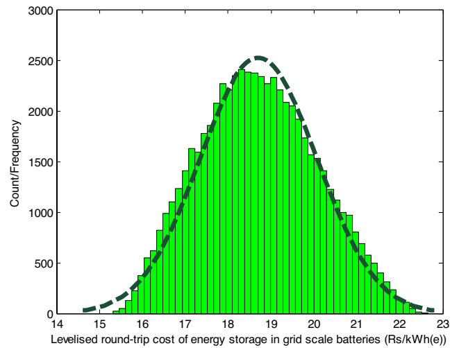
Figure 6 Distribution of levelized round trip cost of electrical energy storage in Vanadium Redox Flow batteries (10 MW, 24-h storage duration)
