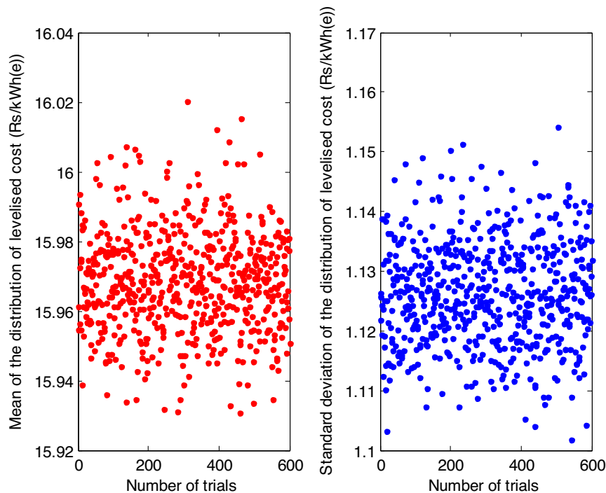
Figure 11 Sampling distributions of mean and standard deviations of levelized round trip cost of electrical energy storage (Li-LFP batteries, 1 MW, 2-h storage)
