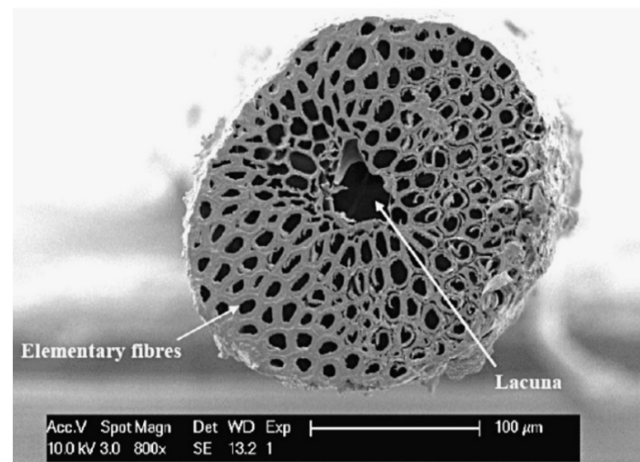
Figure 1 Scanning electron microscope image of cross-sections of a typical coir fiber with lacuna and elementary fibers [12]
