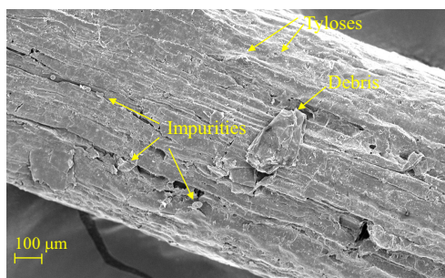
Figure 5 Field emission scanning electron microscopy image of untreated fiber surface at 500 magnification
