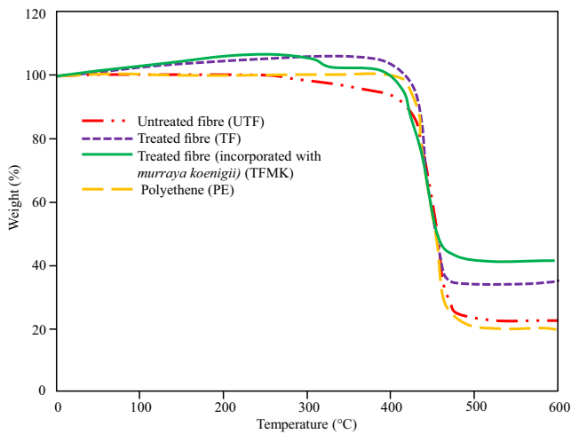
Figure 8 Thermogravimetric of untreated fibers, treated fibers, and treated fibers incorporated with Murraya koenigii
