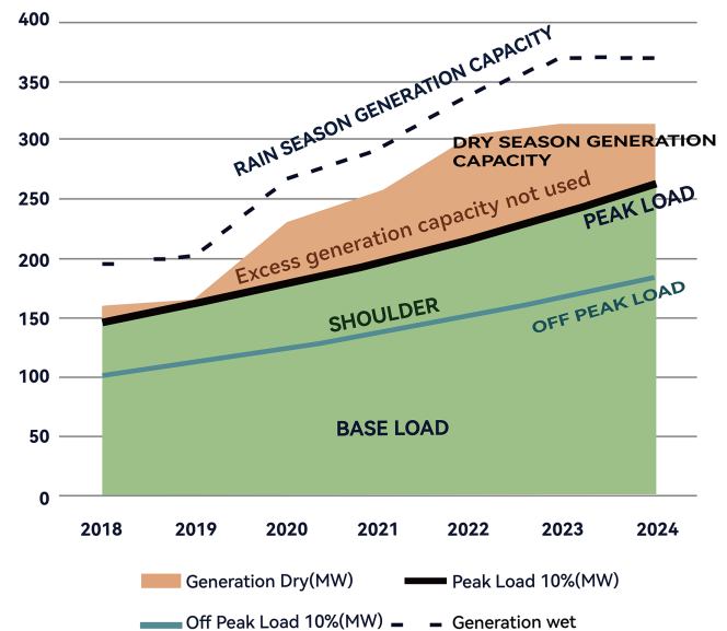
Figure 11 Load balance during the dry season
